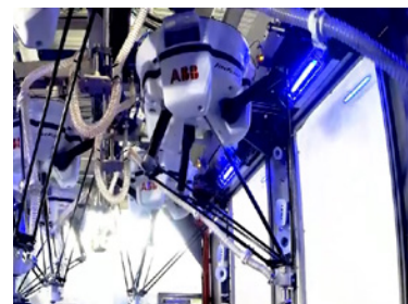
Robot Delta
