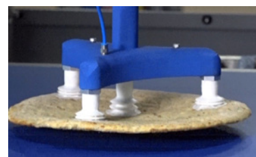
Robot Delta
